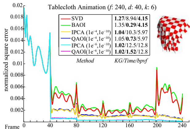
Fig. 10 Observe how fast QAOI reaches the levels of reconstruction quality of IPCA for the entire Tablecloth animation.
