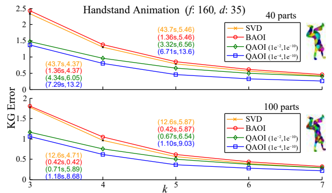
Fig. 8 Approximation as well as time and compression ratio (in brackets) for various k using different spatial clustering on the Handstand animation.
