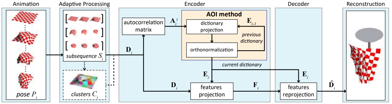
Fig. 4 Our adaptive animation compression pipeline. Temporal, and optionally spatial, clustering is initially employed to support the encoding of sequentially arriving animation frames (left). For each incoming block of frames, the dictionary is estimated by readjusting the subspaces computed at the previous block via adaptive orthogonal iterations (middle). High-quality reconstructions are finally computed by efficiently combining the estimated dictionary and feature vectors (right).
