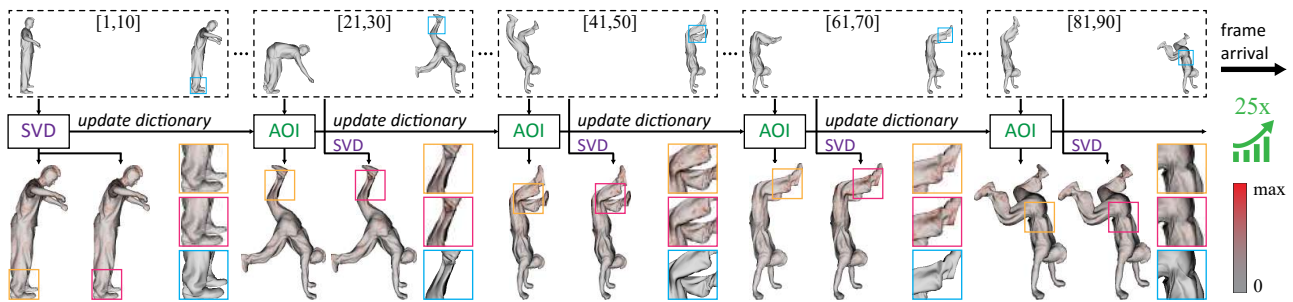
Fig. 1 Overview of our animation compression method. Assuming sequential arrival of the animation data (top), the dictionary is dynamically updated for each cluster (block of 10 frames) by employing adaptive orthogonal iterations (AOI). The reconstructed results of the Handstand animation confirm that AOI achieves similar quality in 25\times faster times when compared to a direct SVD-based solution (bottom).
