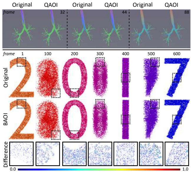
Fig. 9 QAOI (top) and BAOI (bottom) produces high quality visual reproduction despite the extreme temporal incoherence between frame blocks in two particle simulations.
